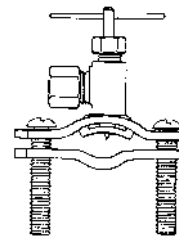
104SCSD Self Drilling Valve Assembly fits 3/8" thru 1-3/8" O.D. Copper Tubing
